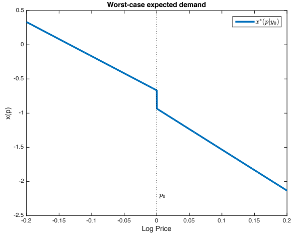
(a) No restrictions on admissible m(p)
