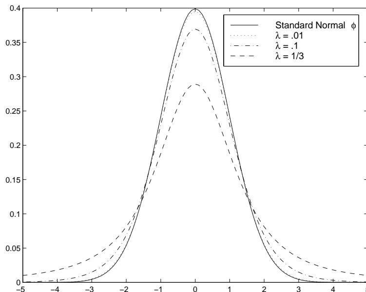
Figure 1: h_{\lambda,0} and the normal density
