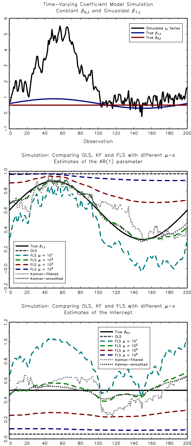
Figure 3: The ability of FLS and the Kalman-filter to capture sinusoid change in \beta_{1,t}
