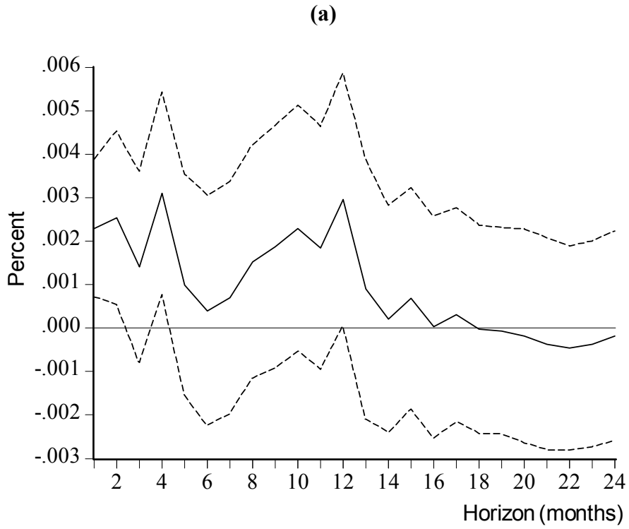
Figure 8 GIRs of \pi - \pi^* to one S.D. shock in the equation for the (a) (e - e^*) , (b) REXR , and (c) \Delta \tilde{m} with Monte Carlo standard errors Mexico, 1991.1-2001.6
