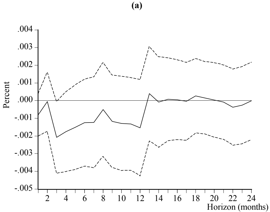
Figure 7 GIRs of \pi - \pi^* to one S.D. shock in the equation for (a) (\tilde{m} - \tilde{m}^*) and (b) HPF(y - y^*) with Monte Carlo standard errors Chile, 1992.6-2001.6
