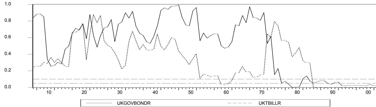
Figure 1: Granger-causality p-values: Rolling Regressions (30 years window)
