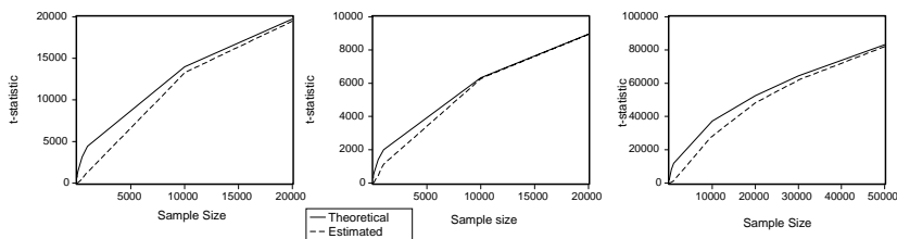
Graphs of t -statistics based on Theorem 1 and simulated data. Left panel: \lambda_y = 0.55, \lambda_x = 0.45 ; middle: \lambda_y = 0.75, \lambda_x = 0.25 ; right: \lambda_y = 0.95, \lambda_x = 0.05 ; all panels: \beta_y = \beta_x = 0.2, \gamma_y = \gamma_x = 0.02 .
