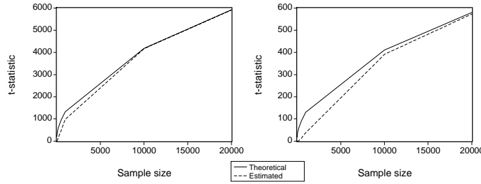
Graphs of t -statistics based on Theorems 3 and 4 and simulated data. Left panel based on regression model (1), while right panel based on model (4). Both panels:
