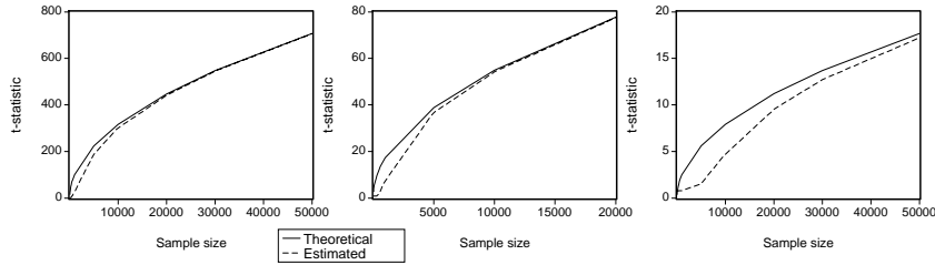
Graphs of t -statistics based on Theorem 2 and simulated data. Left panel: \lambda_y = 0.55, \lambda_x = 0.45 ; middle: \lambda_y = 0.75, \lambda_x = 0.25 ; right: \lambda_y = 0.95, \lambda_x = 0.05 ; all panels: \beta_y = \beta_x = 0.2, \gamma_y = \gamma_x = 0.02 .
