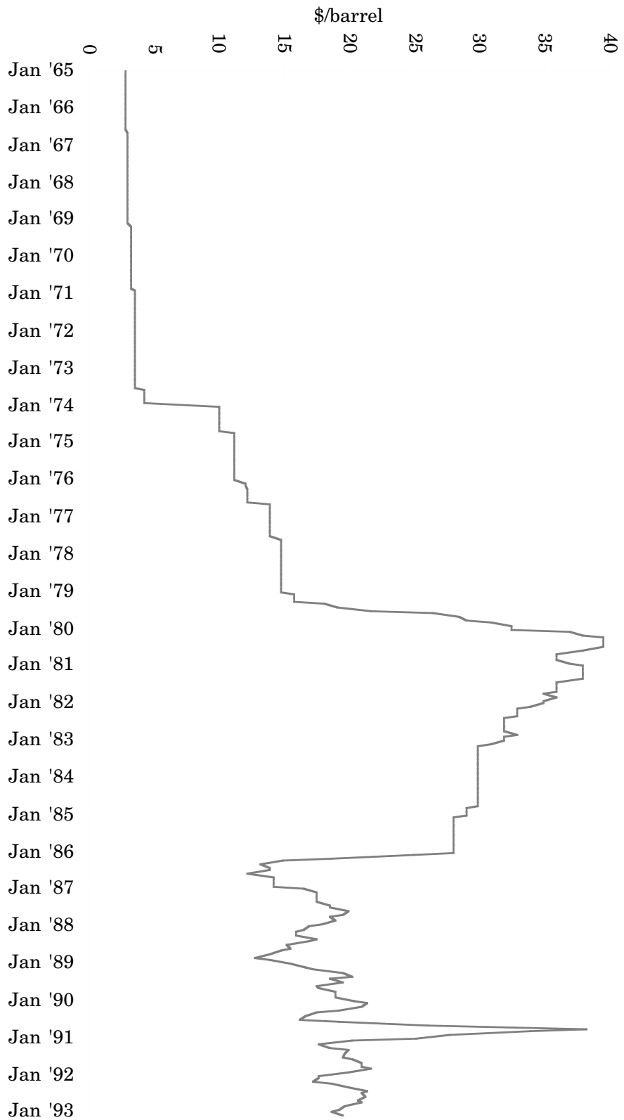
Figure 1 - Price of Oil
