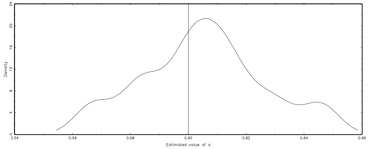
Figure 3: Density for PMLE estimates from 500 Monte Carlos and 100 obs
