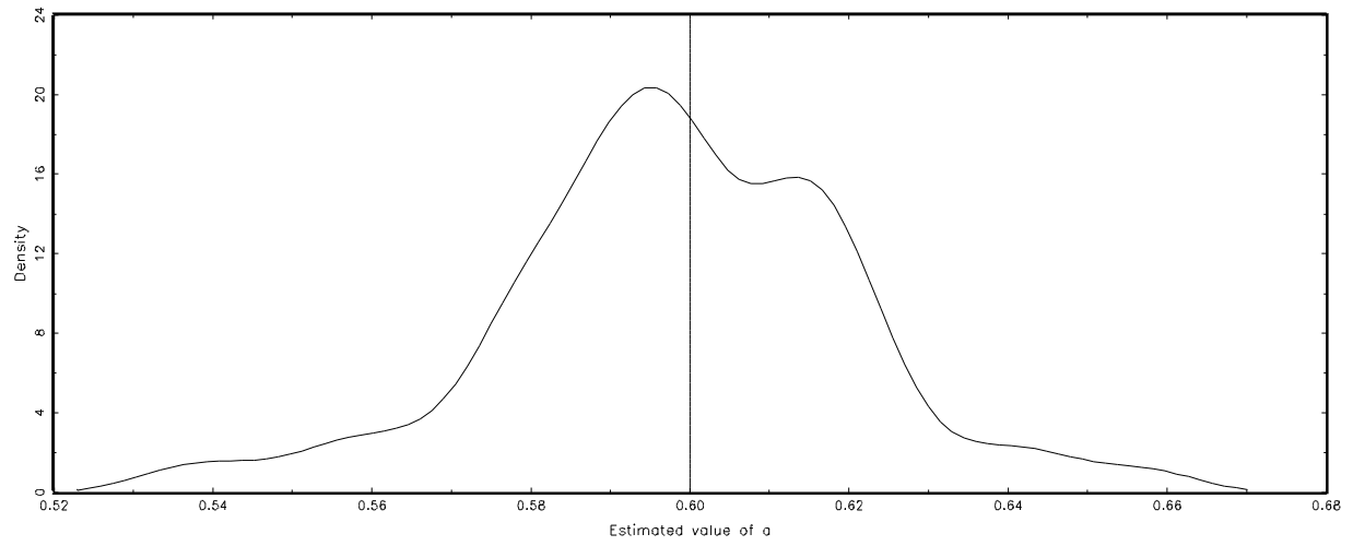
Figure 4: Density for PMLE estimates from 500 Monte Carlos and 200 obs
