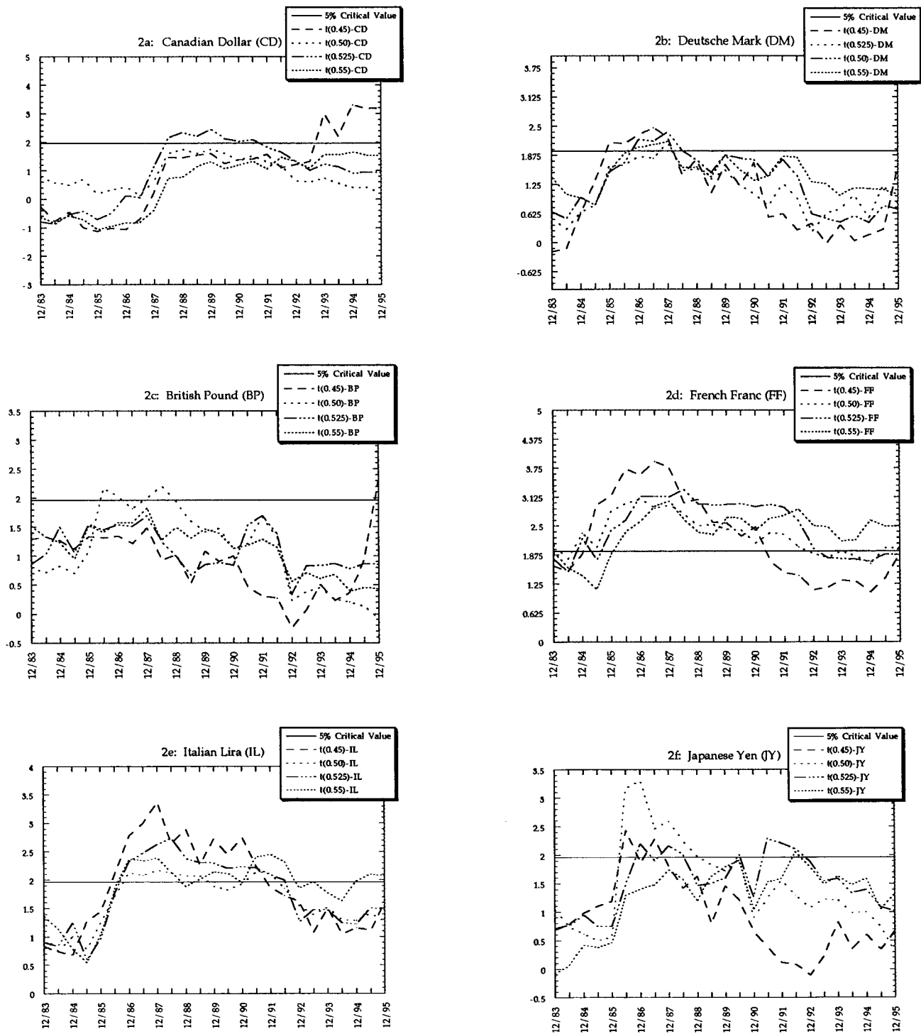
Figure 2: t-statistics for the Gaussian Semiparametric d Estimates over Subsamples
