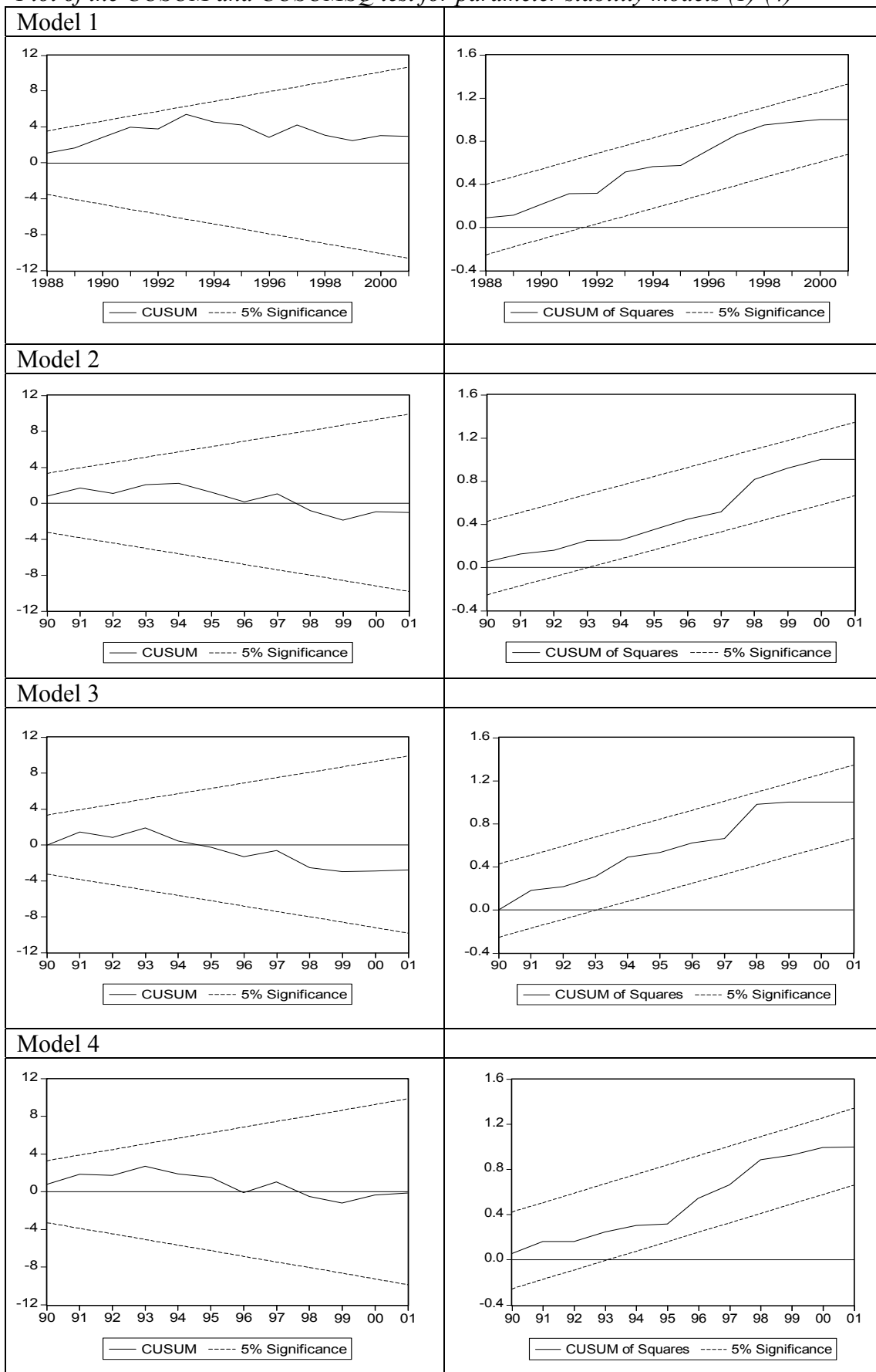
Figure 1. Plot of the CUSUM and CUSUMSQ test for parameter stability models (1)-(4)
